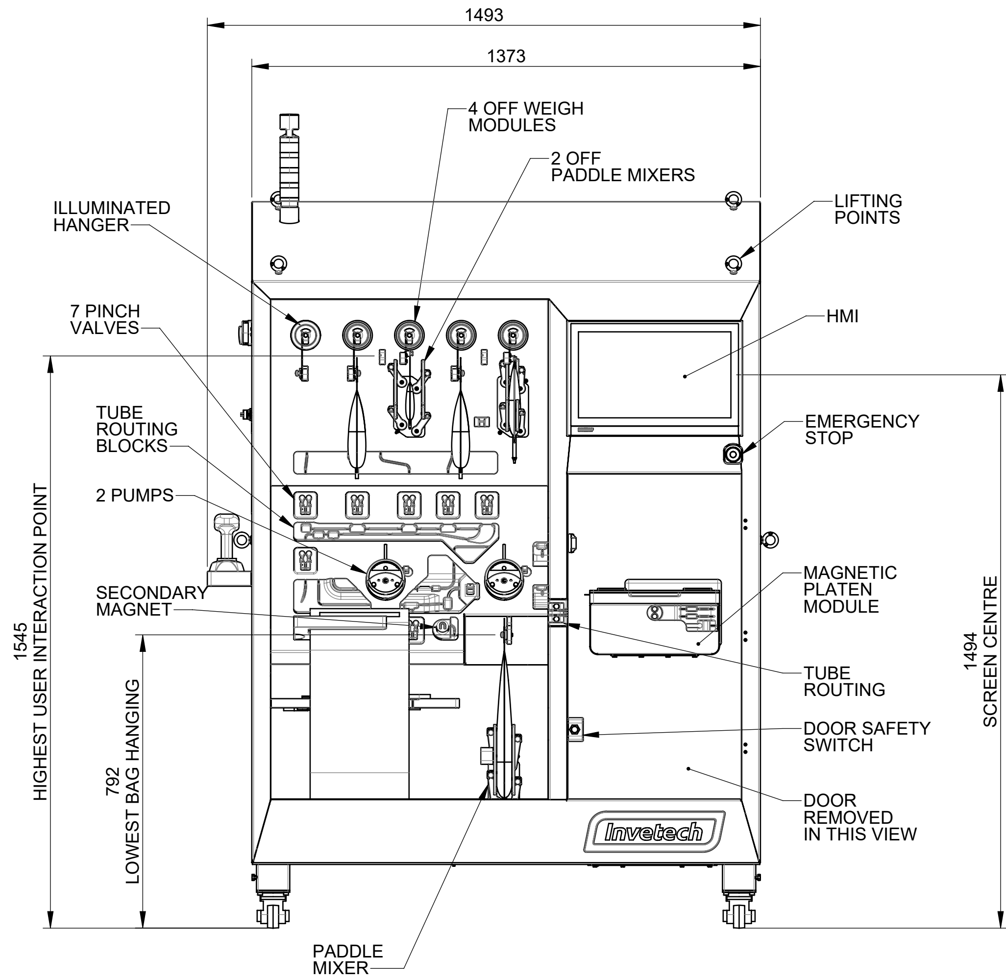
FRONT VIEW
