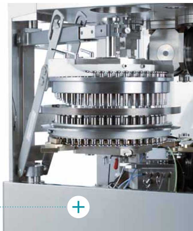
Dismantling arm with segment turret
